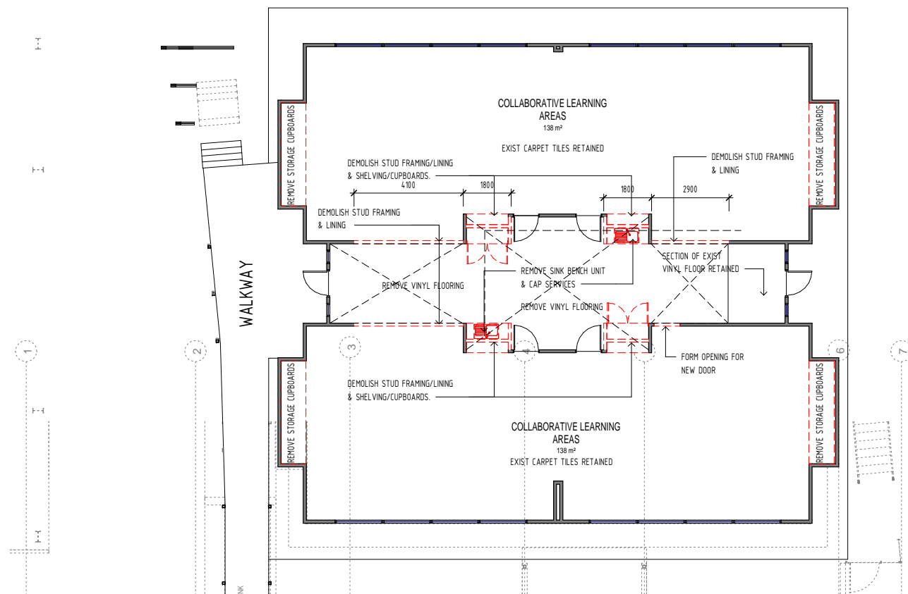
2 TENISON WOODS BUILDING - PLAN - DEMOLITION FIRST FLOOR PLAN 1 : 100
