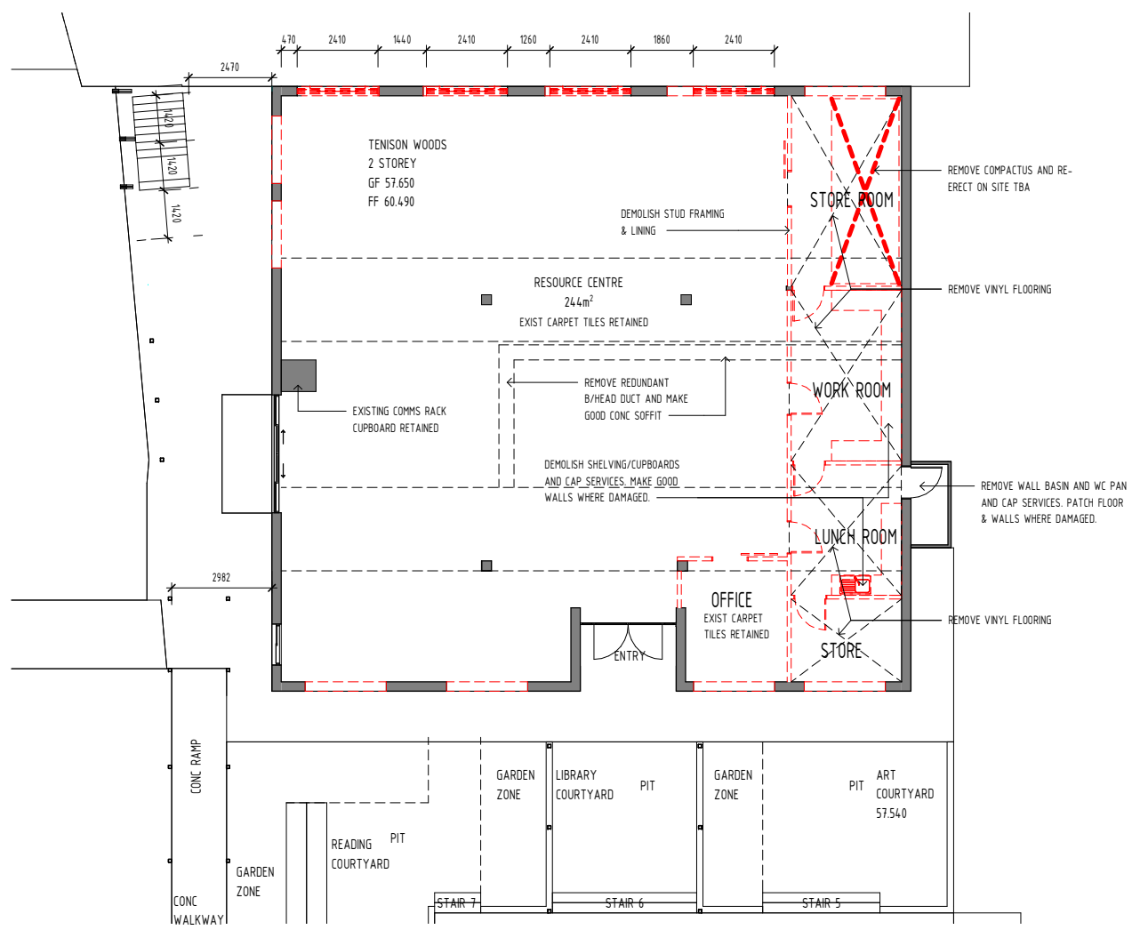
1 TENISON WOODS BUILDING - PLAN - DEMOLITION GROUND FLOOR 1 : 100
